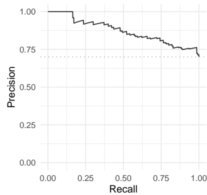
Figure 3.12: Precision-Recall curve based on tsk("german_credit") and lrn("classif.ranger") .
